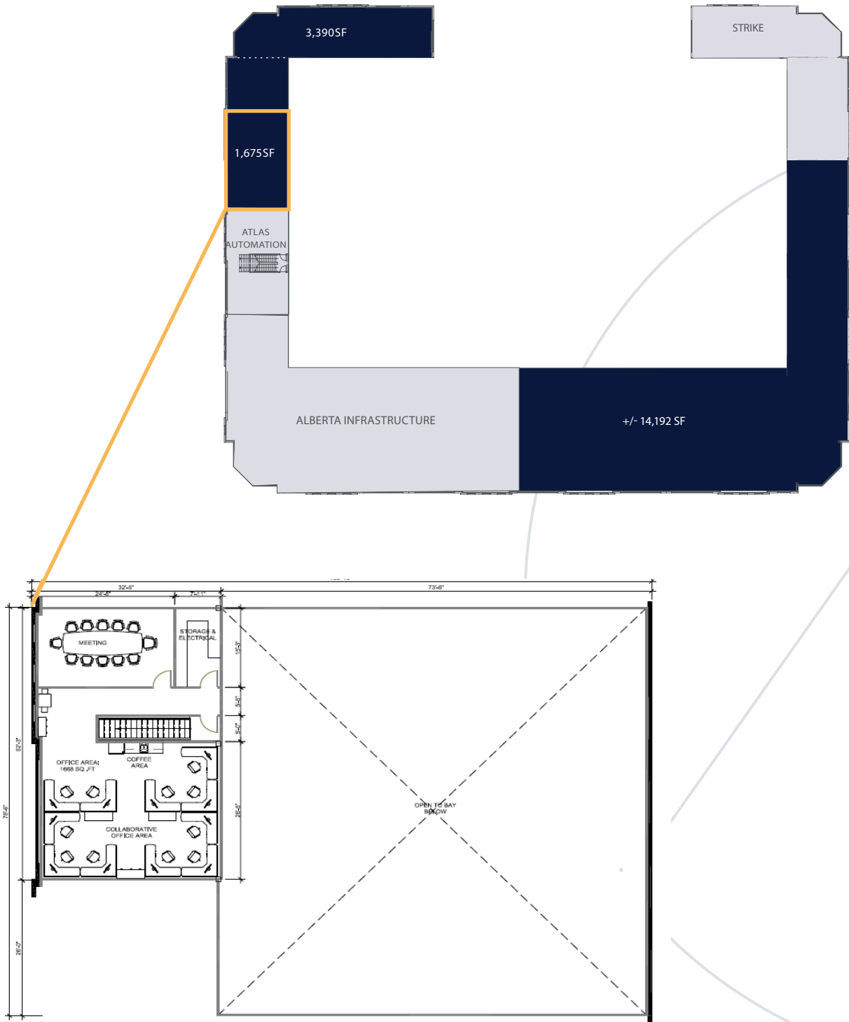
SECOND FLOOR Conceptual Plan, 4'x4' Design Grid
