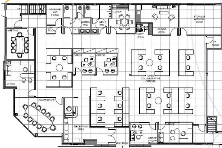
MAIN FLOOR Conceptual Plan, 4'x4' Design Grid
